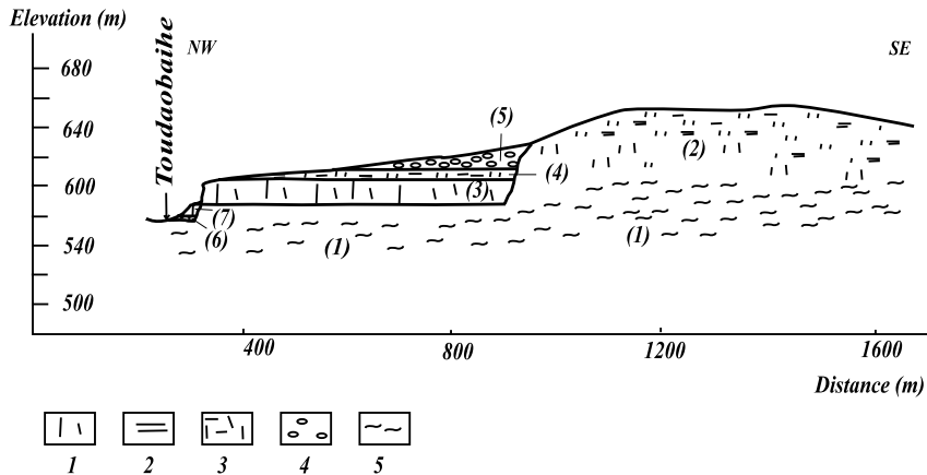
Fig. 2 The Yaoshui profile for the basalt sequence of the Toudao Formation
