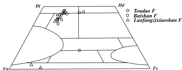
Fig. 4 Pyroxene compositional differences between the different stages of the Shield Basalts
