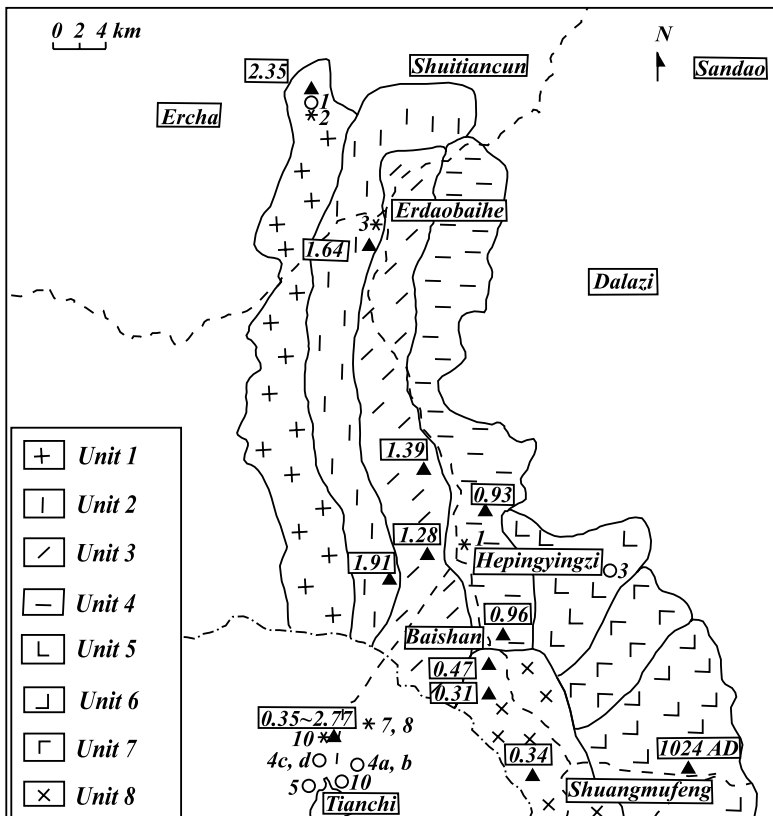
Fig. 5 Schematic distribution of the northeast lava flows of the Tianchi Volcano.
