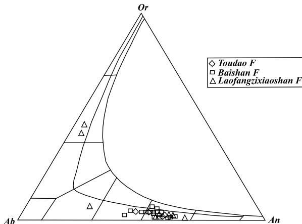
Fig. 6 Or-Ab-An plots of feldspar in shield-forming eruptions.
